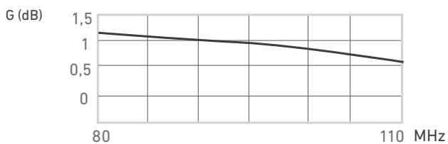
Gain diagram
