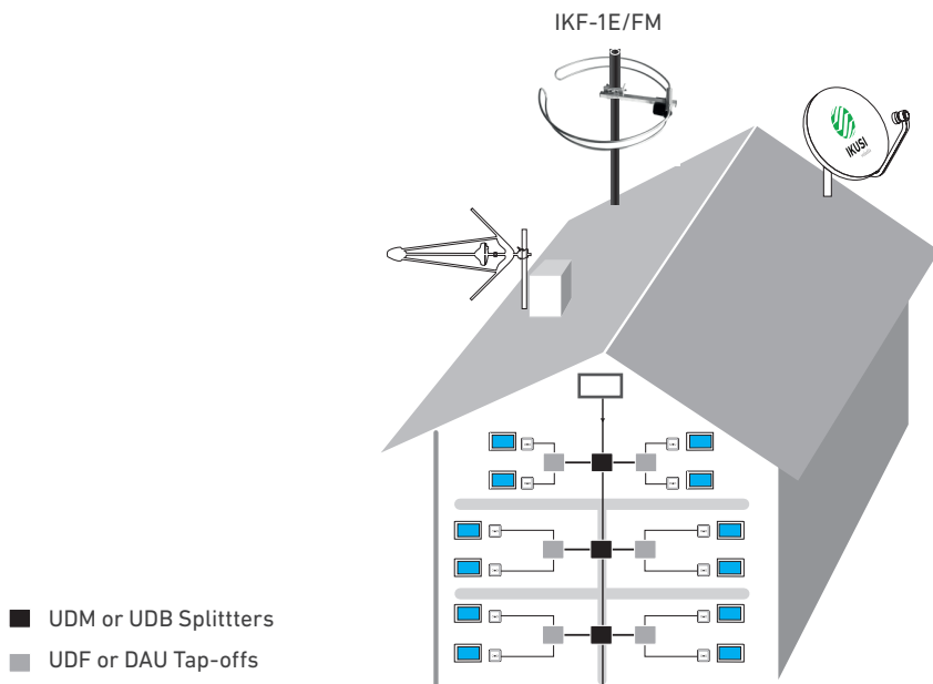
Installation example
